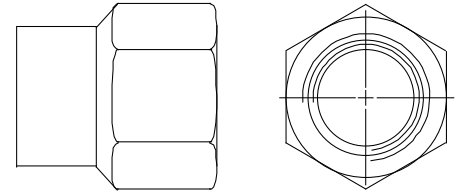
Figure 3: Brass adapter G 3/8 female to 1/4-18 NPT female
